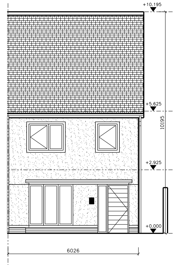
FRONT ELEVATION
